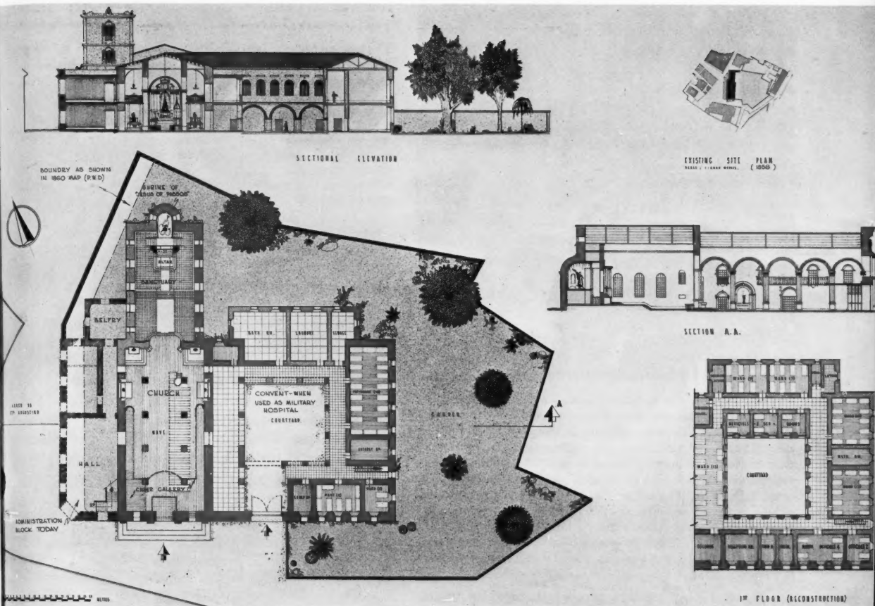
Fig. 1. Plans, sections, and site plan, Monastery of St. Augustine, Macao, at the present time.
